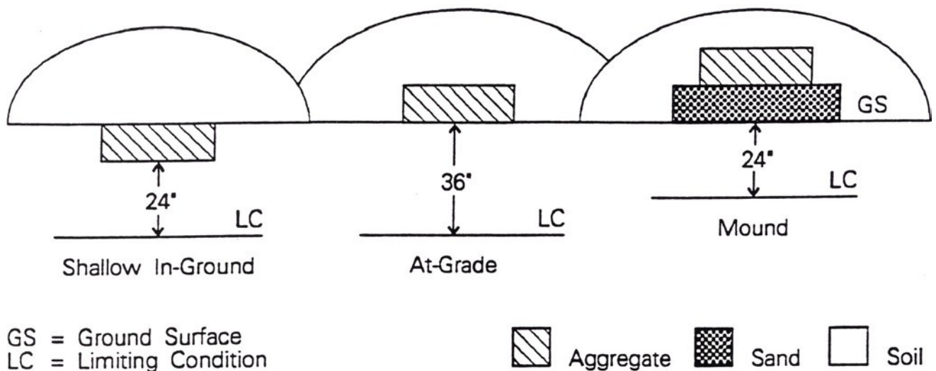
Figure 13.4a SIG (requires pretreatment), At-Grade, Mound Soil Below Trench Bottom Requirements
