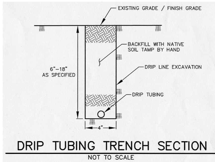
Figure 13.6a – Drip Trench Cross-Section
