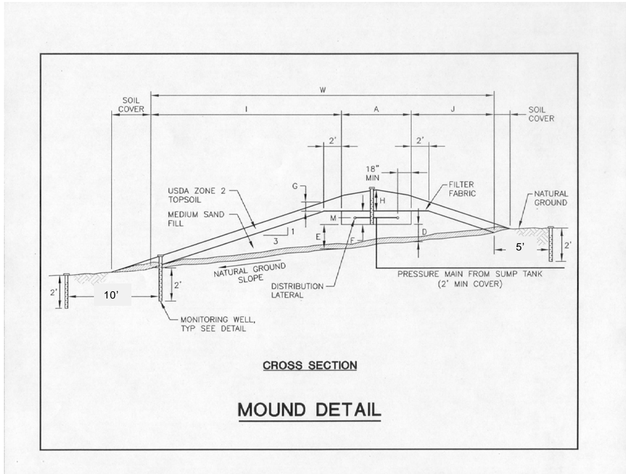
Figure 13.3b – Mound Cross Section
