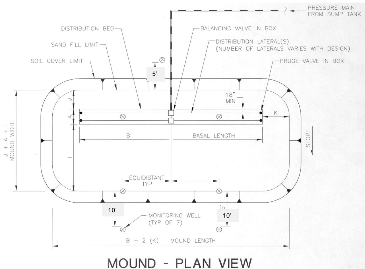
Figure 13.3c – Mound Plan View
