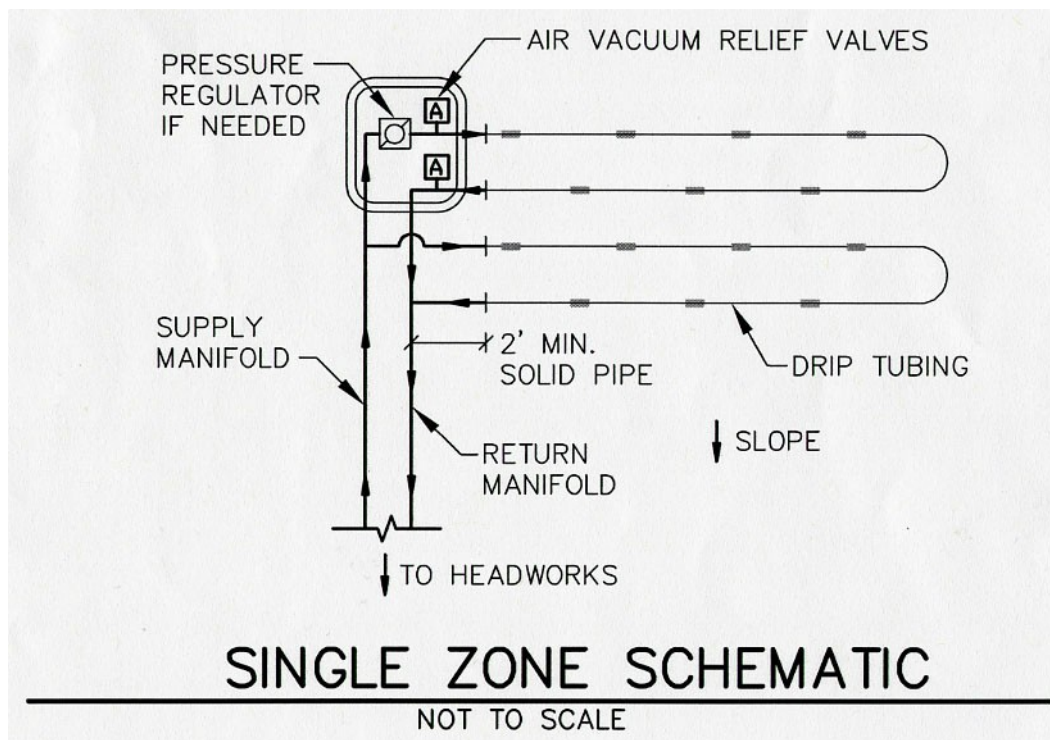
Figure 13.76b – Example Single Zone Schematic
