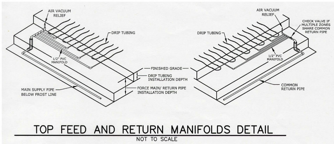
Figure 13-76d Example Manifold Connection
