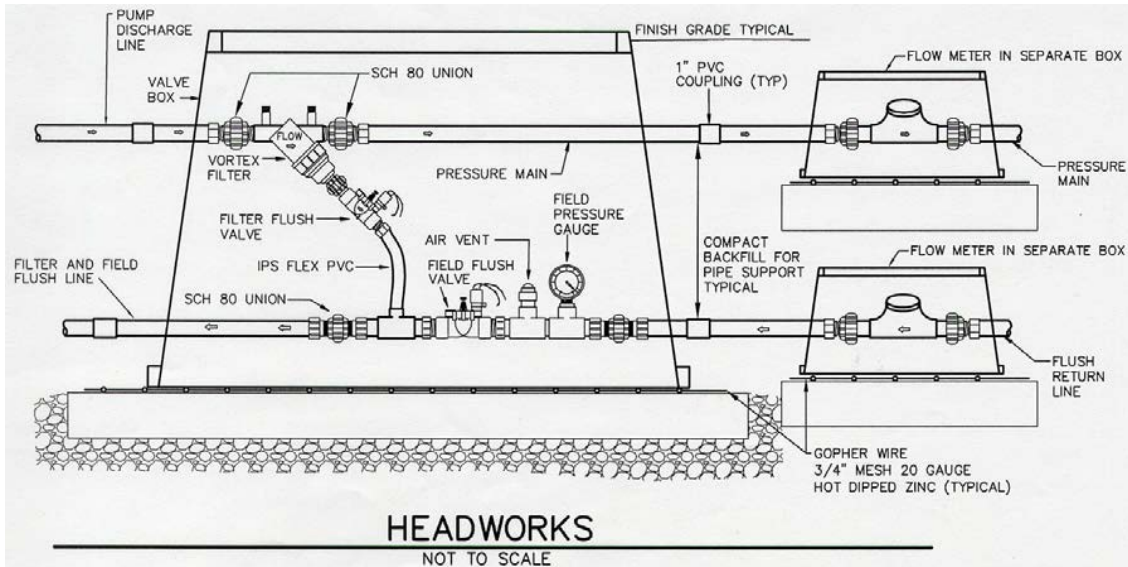
Figure 13.-76f – Example Headworks
