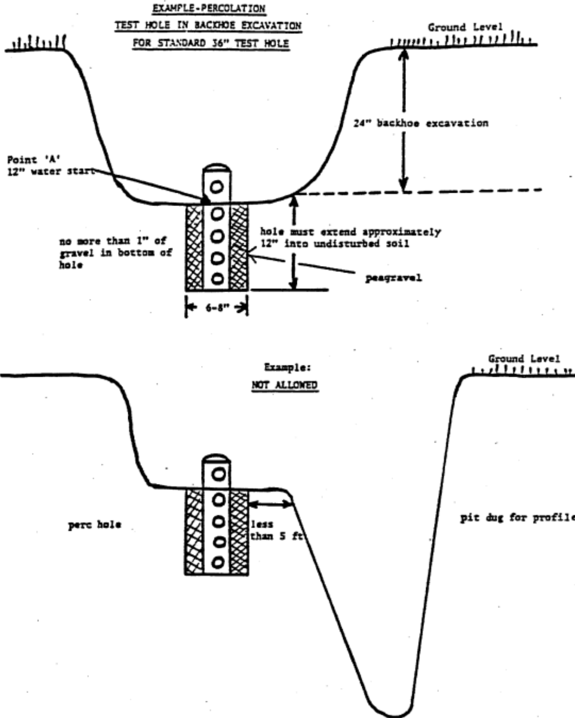
Figure 7.8b Percolation Test Hole
