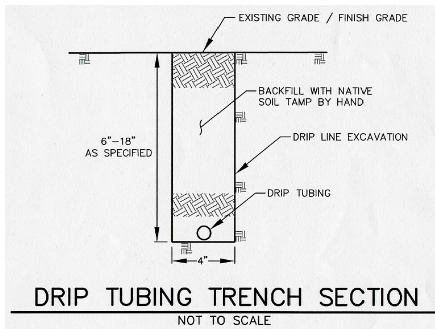
Figure 13.-76a – Drip Trench Cross-Section
