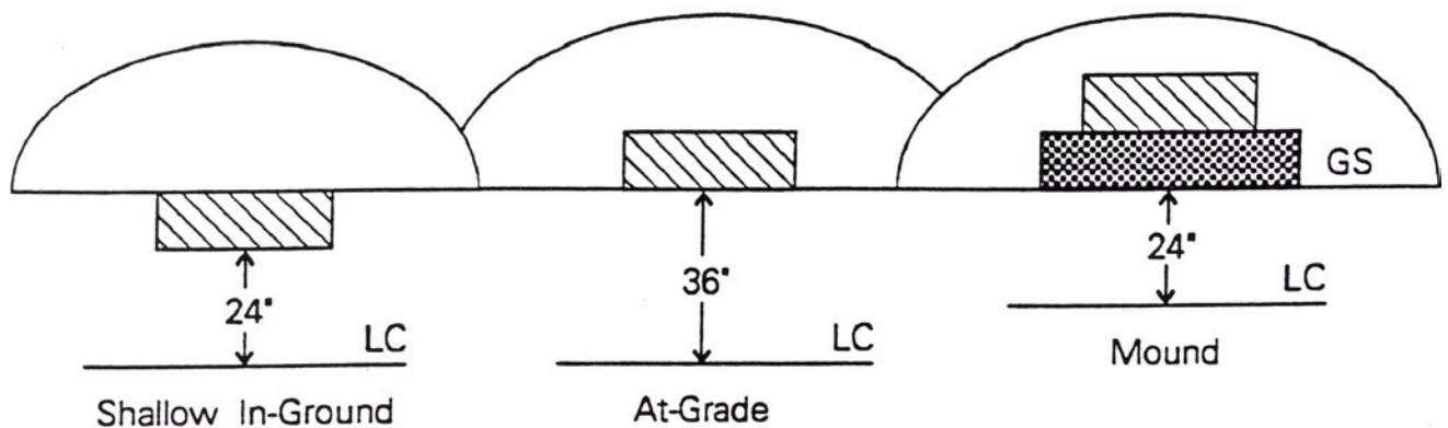
Figure 13.45a SIG (requires pretreatment), At-Grade, Mound Soil Below Trench Bottom Requirements
