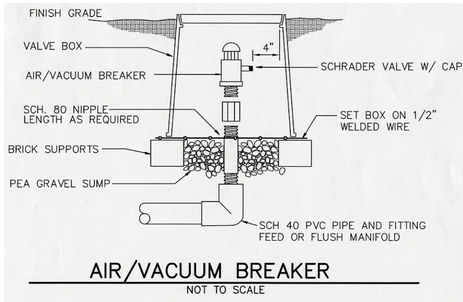
Figure 13.-76e – Example Air Relief with Schrader Valve
