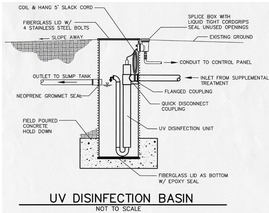
Figure 13.76g – Example Disinfection Unit
