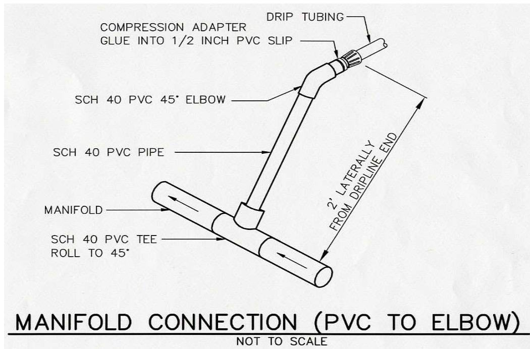
Figure 13.6d Example Manifold Connection
