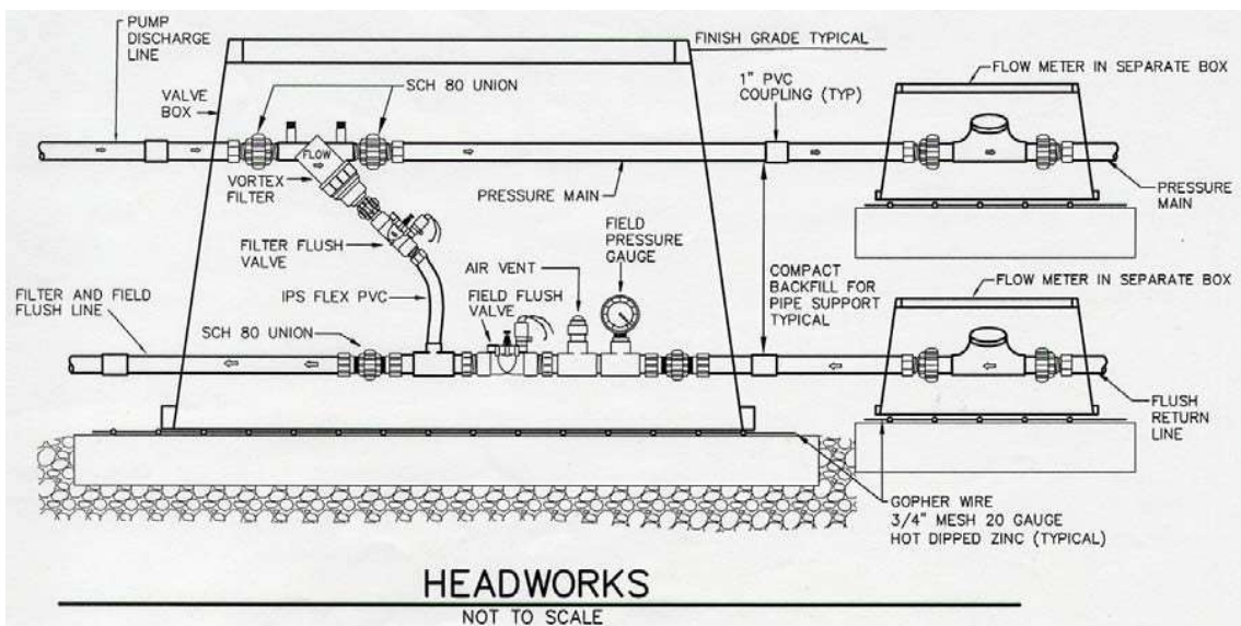
Figure 13.6f – Example Headworks
