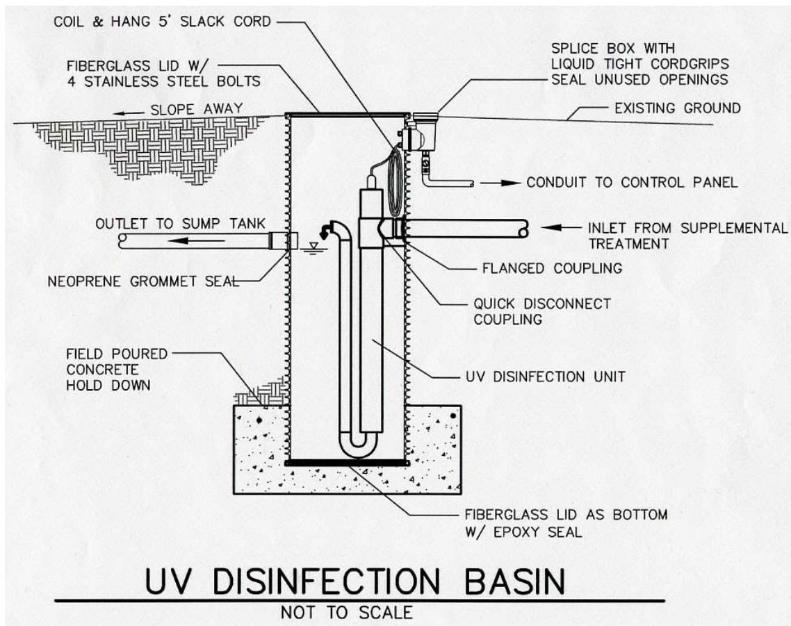
Figure 13.6g – Example Disinfection Unit
