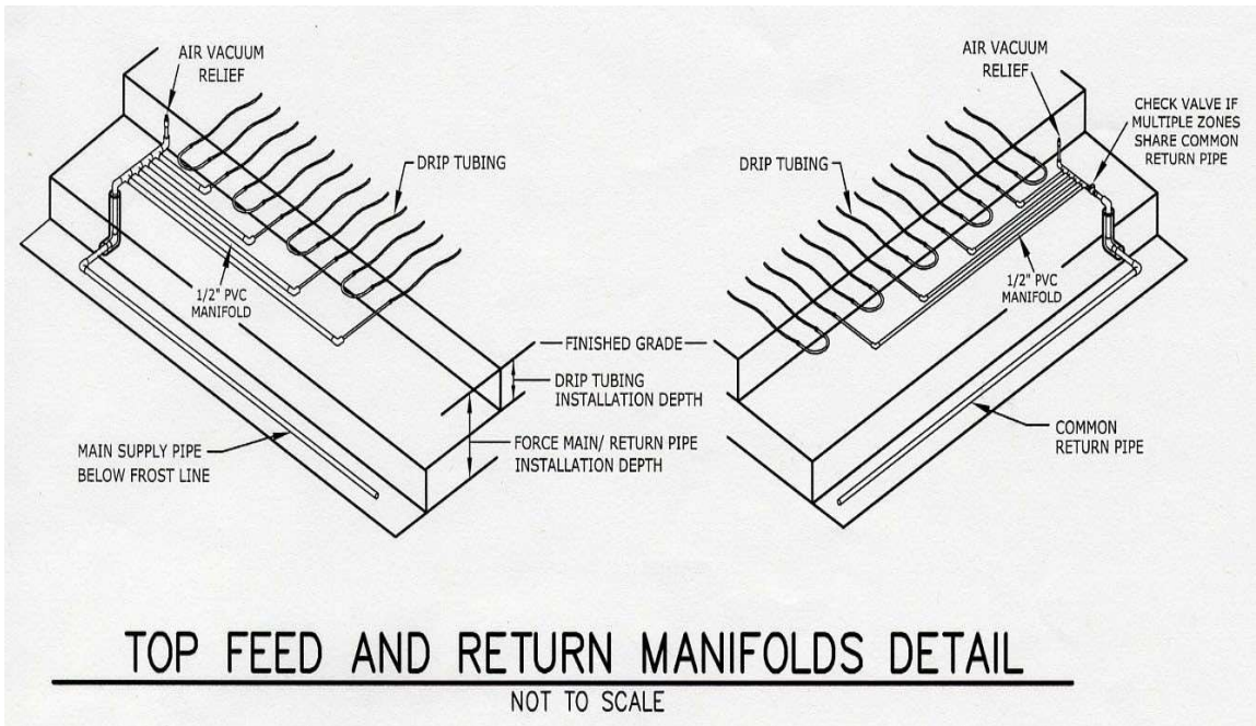
Figure 13.6c – Example Top Feed Manifold
