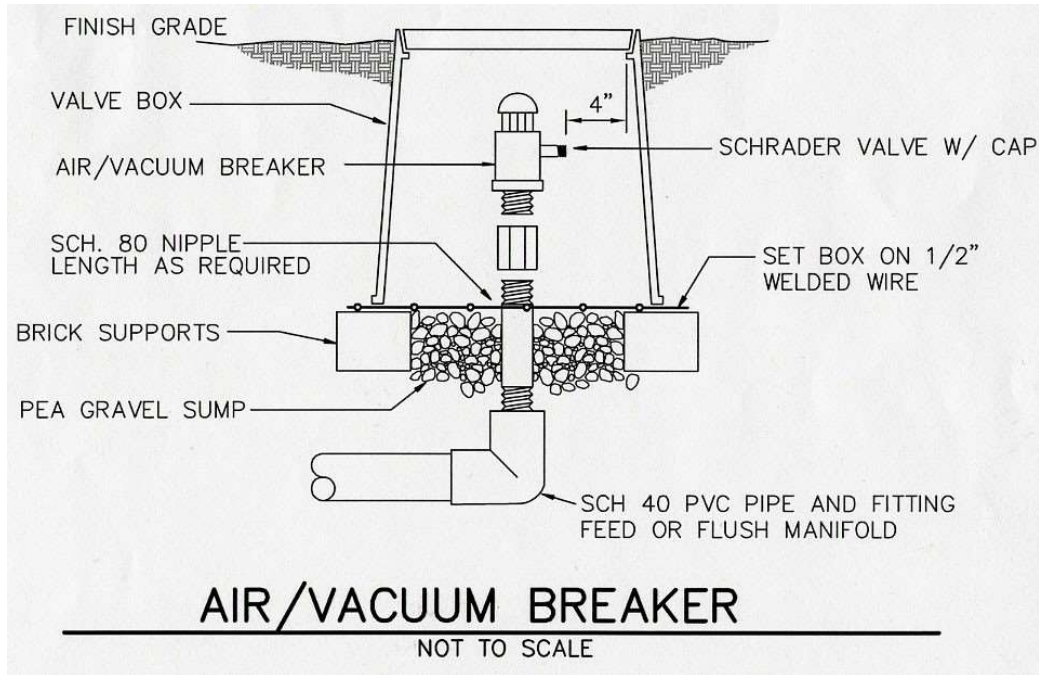
Figure 13.6e – Example Air Relief with Schrader Valve
