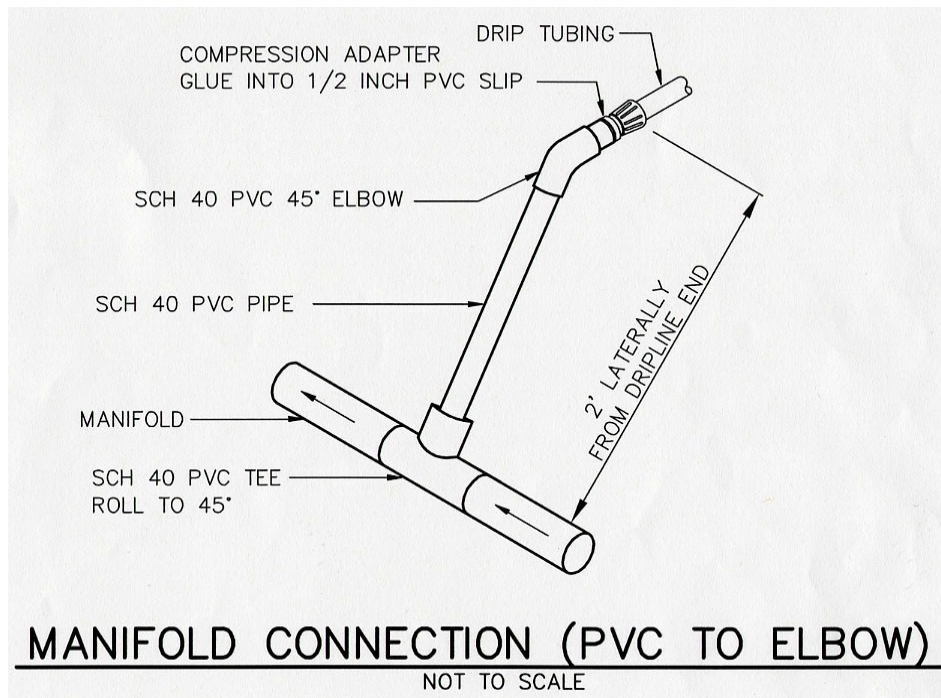
Figure 13.7d Manifold Connection
