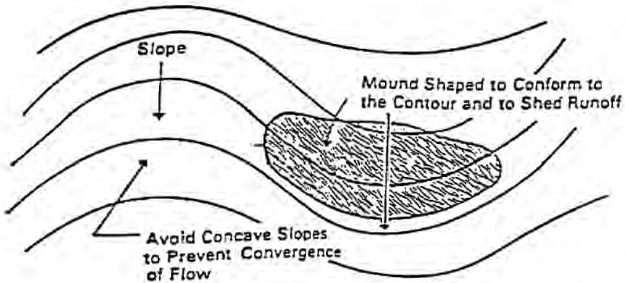
Figure 13.3e – Contour Conformance
