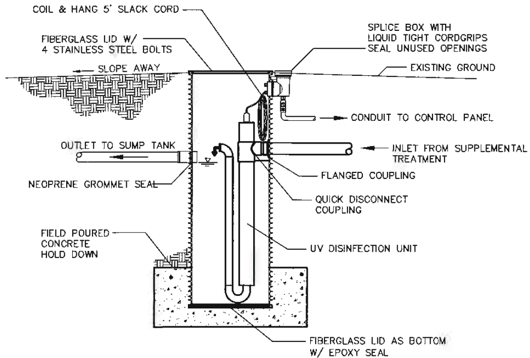
Figure 13.7g – Example Disinfection Unit
