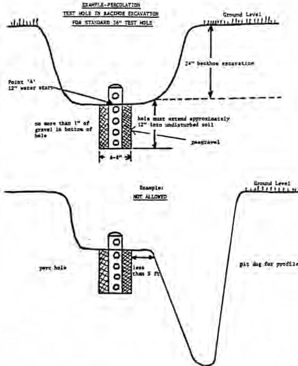
Figure 7.8b Percolation Test Hole
