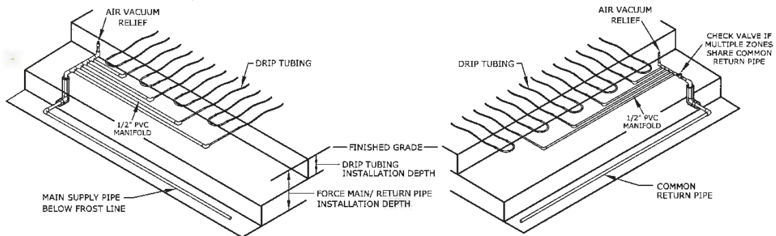
Figure 13.7c – Example Top Feed Manifold
