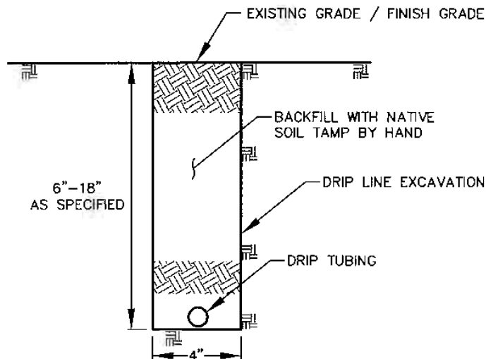
Figure 13.7a – Drip Trench Cross-Section
