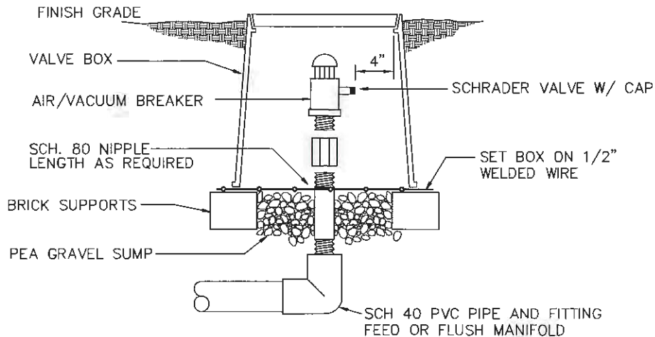
Figure 13.7e – Example Air Relief with Schrader Valve
