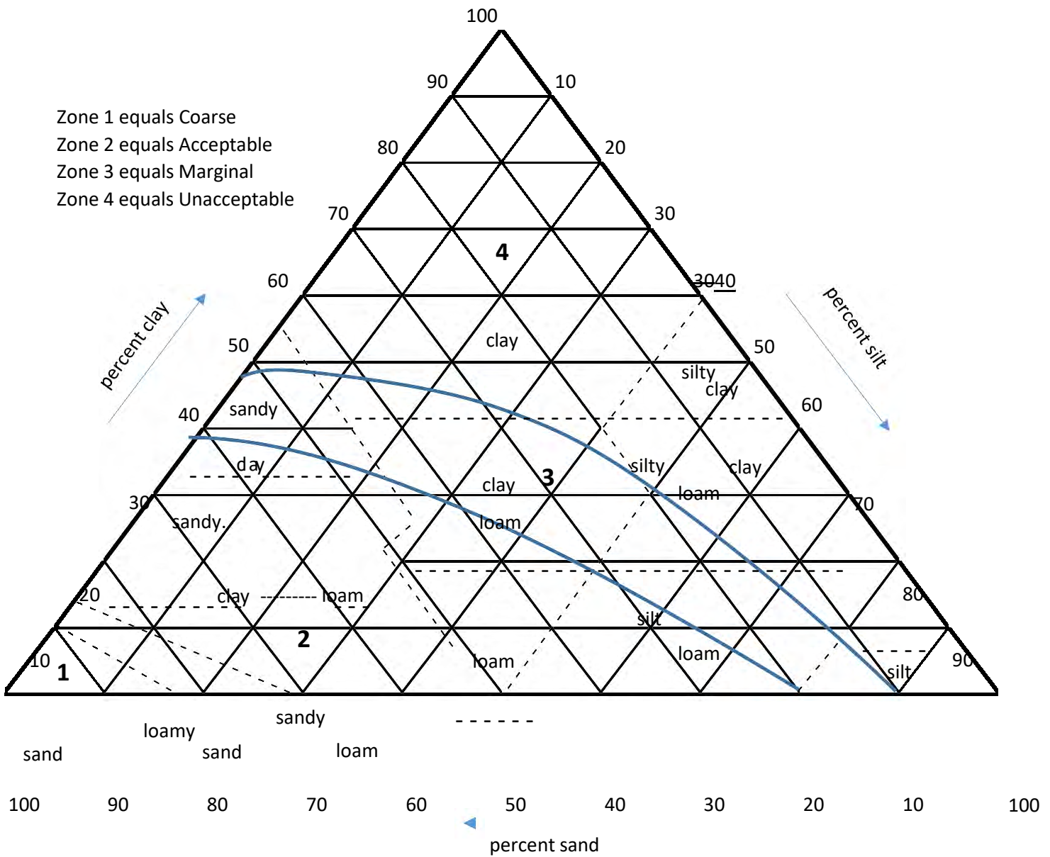
Figure 7.4 Soil Percolation Suitability Chart for OWTS
