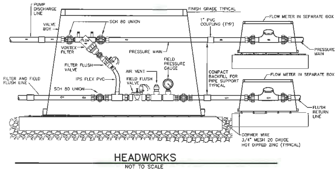
Figure 13.7f – Example Headworks
