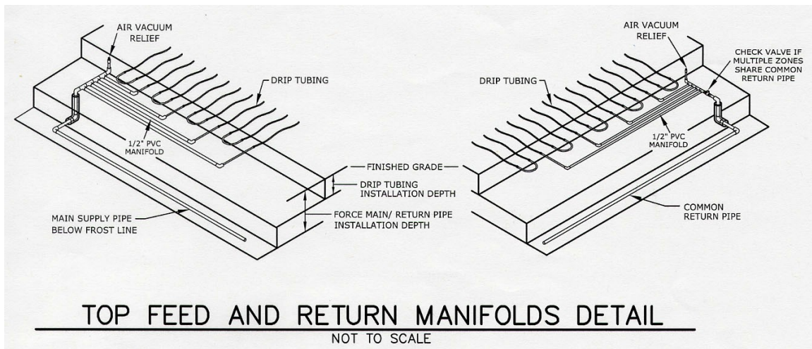
Figure 13.7d Manifold Connection
