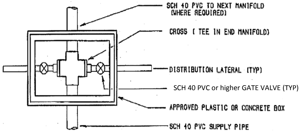
PLAN VIEW BALANCING VALVE DETAIL
