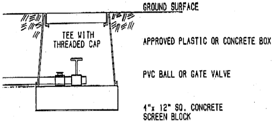
PURGE VALVE DETAIL NTS
